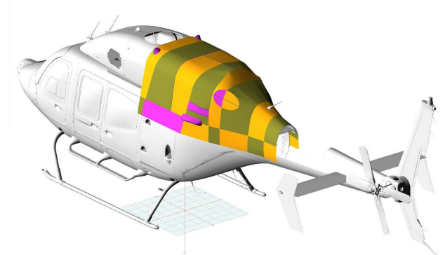
Bell 429 Aft Engine Area Cover, 3D model
