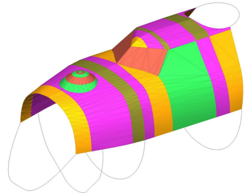
Boeing B-17 Extended Canopy Cover, 3D model
