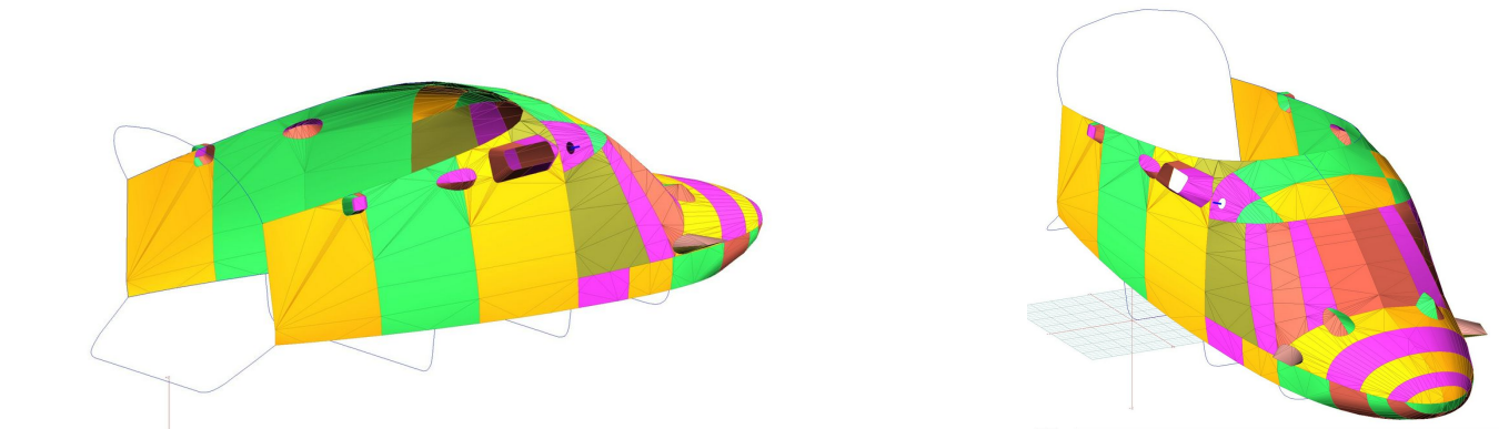
Agusta Leonardo A169 Bubble Cover with Wire Strike, 3D model Agusta Leonardo A169 Bubble Cover with Wire Strike, 3D model
