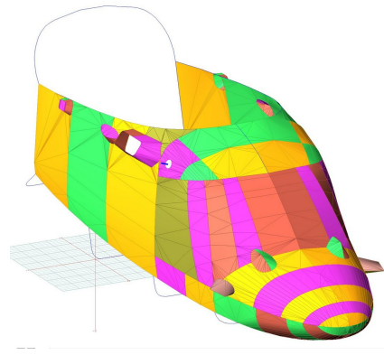
Koala Bubble, Rotor Hub, Blade & Tail Rotor Covers (illustration) Agusta Leonardo A169 Bubble Cover with Wire Strike, 3D model
